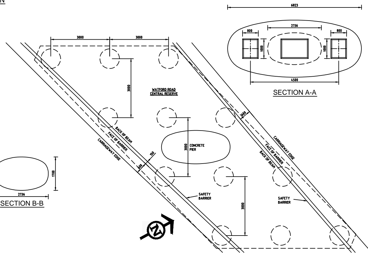
PLAN ON PIER No.5 - FIXED BEARING PIER WITHIN WATFORD ROAD TRAFFIC ISLAND
