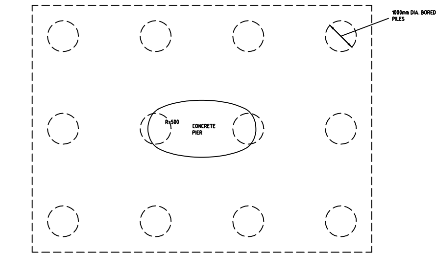
PLAN ON PIER Nos. 1 TO 4 AND 6 TO 8
